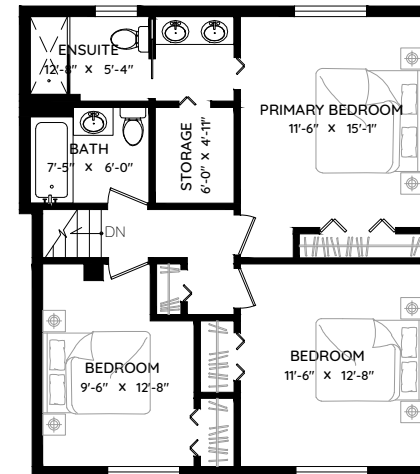
UPPER FLOOR 754 SQ.FT. CH: 8'-0"
